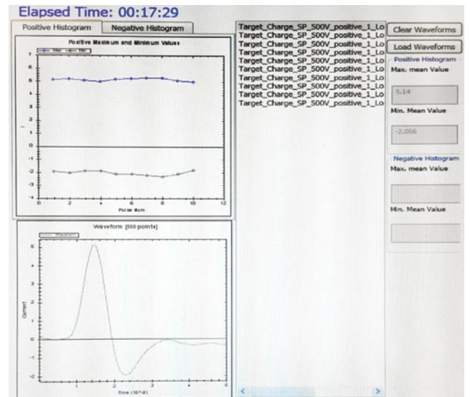
10 Positive 500 V pulse verifications with test target
