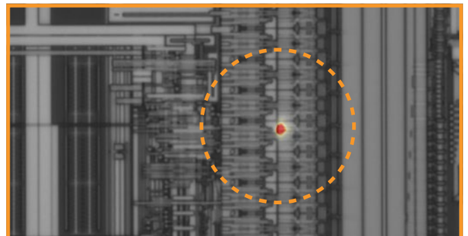
Hotspot observed on the device
