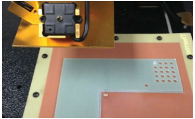
Device on charging plate with alignment tool
