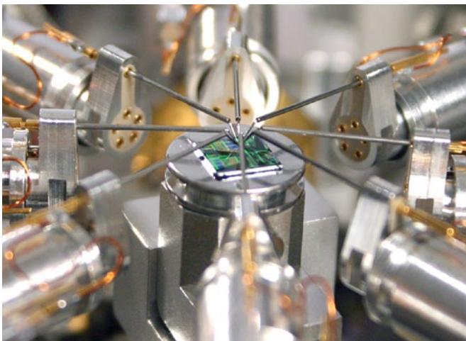
Nanoprober
