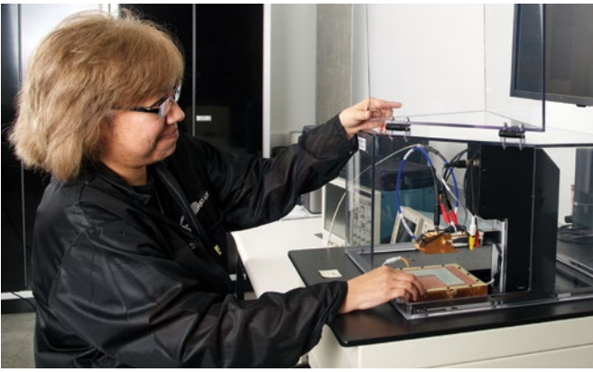
The standard CDM ESD stress setup
