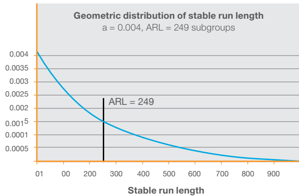
Figure 1 Run length distribution for the Xbar and S scheme
